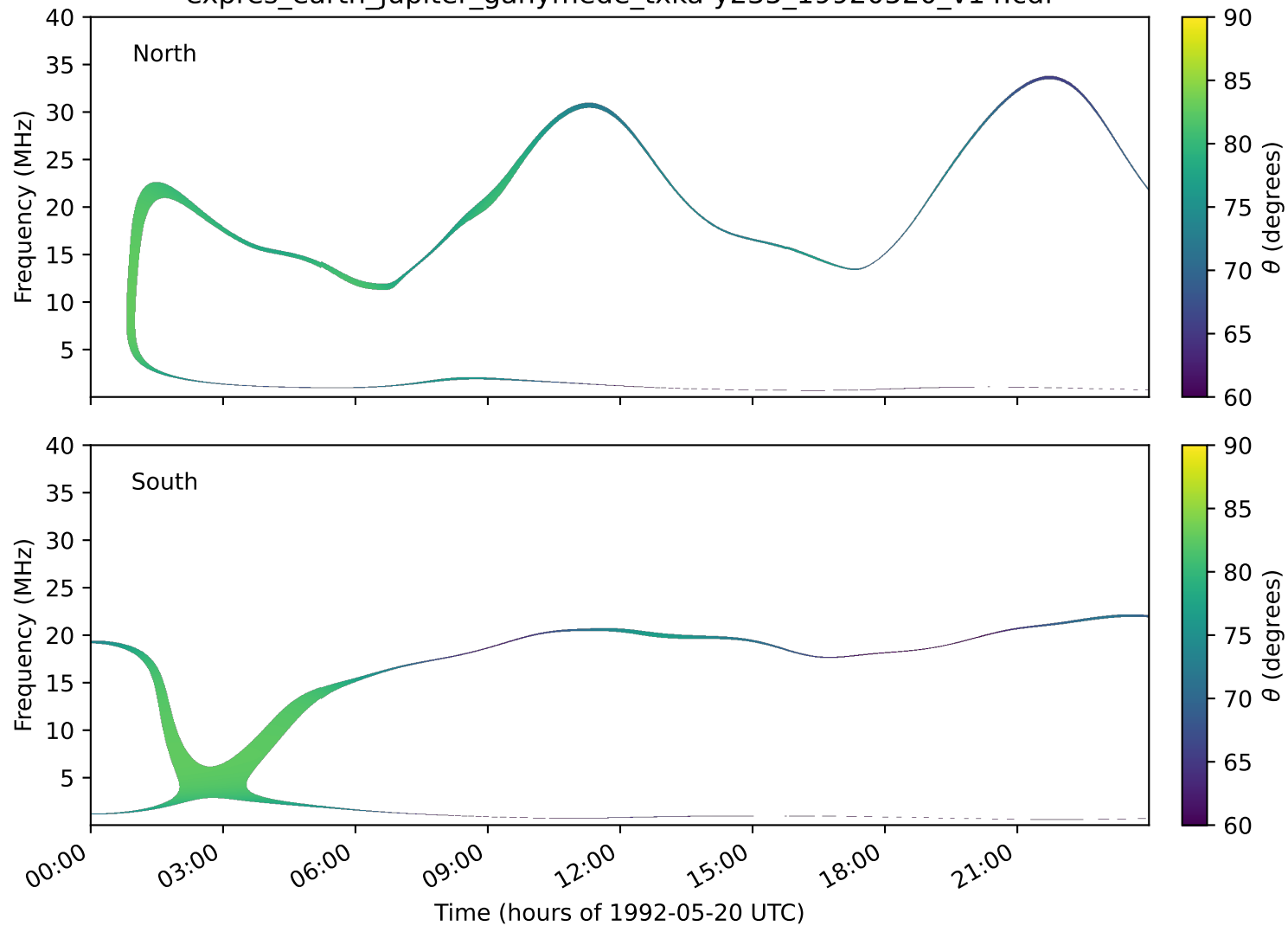
expres_earth_jupiter_ganymede_txka-y235_19920520_v14.cdf
