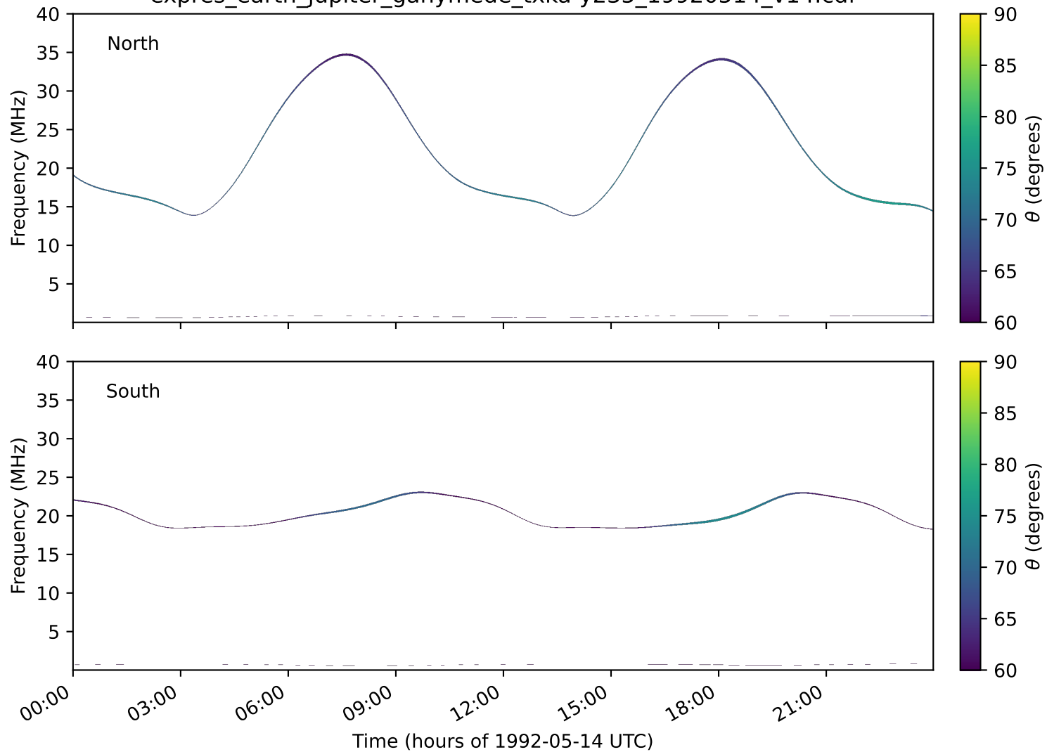
expres_earth_jupiter_ganymede_txka-y235_19920514_v14.cdf
