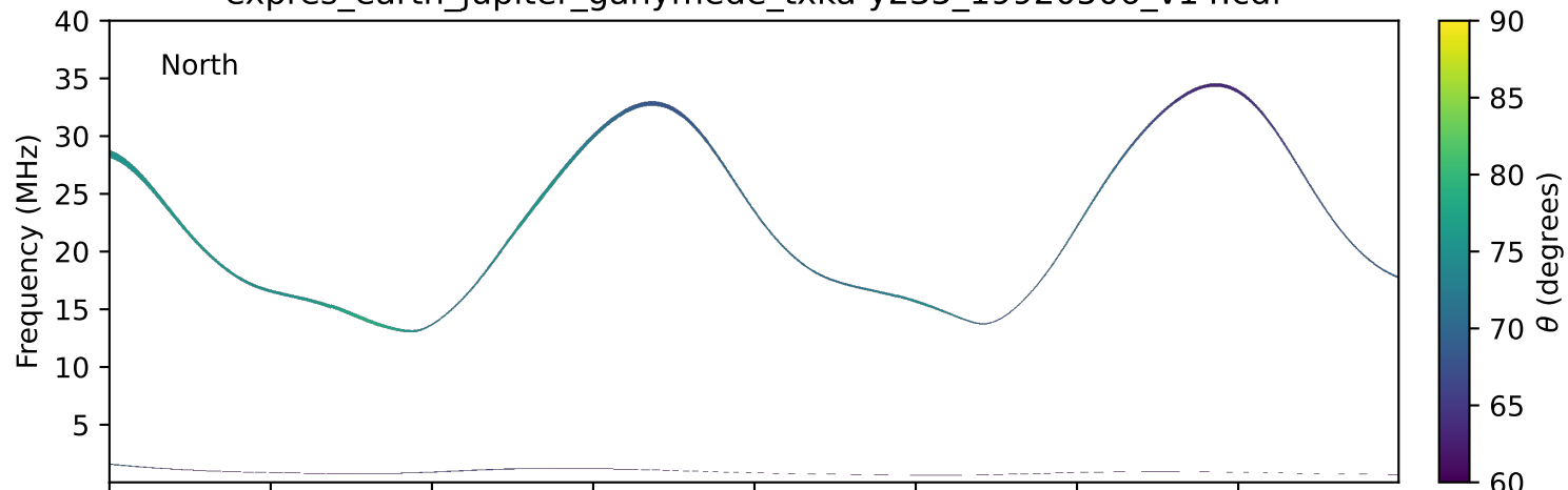
expres_earth_jupiter_ganymede_txka-y235_19920506_v14.cdf
