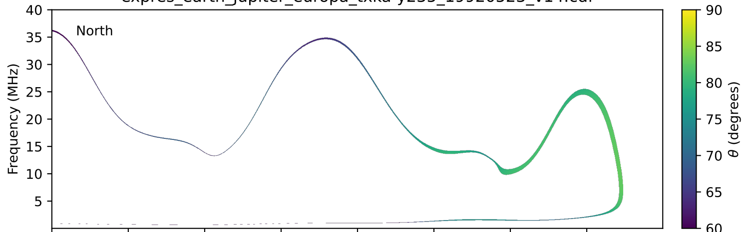
expres_earth_jupiter_europa_txka-y235_19920523_v14.cdf
