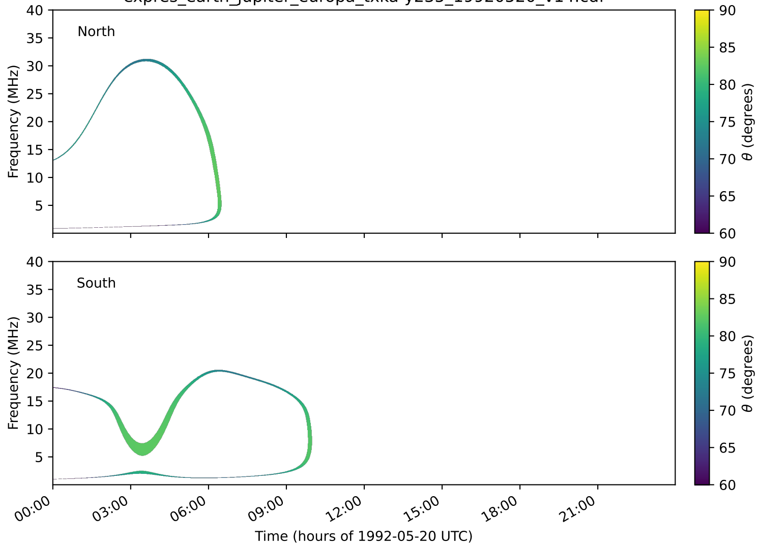
expres_earth_jupiter_europa_txka-y235_19920520_v14.cdf
