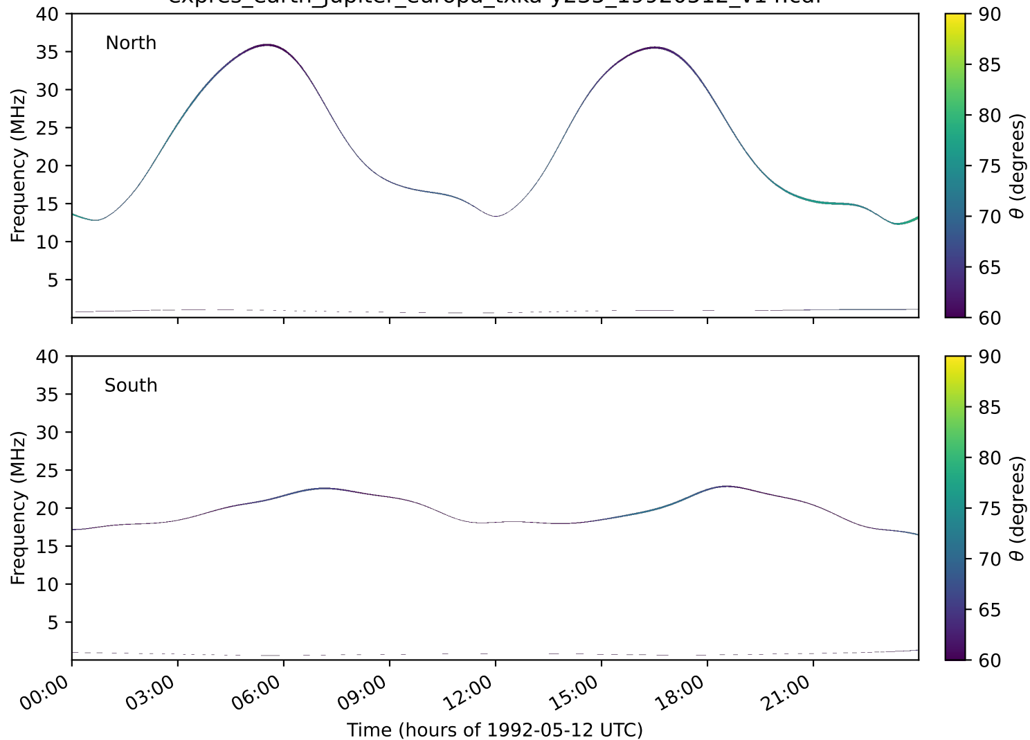
expres_earth_jupiter_europa_txka-y235_19920512_v14.cdf
