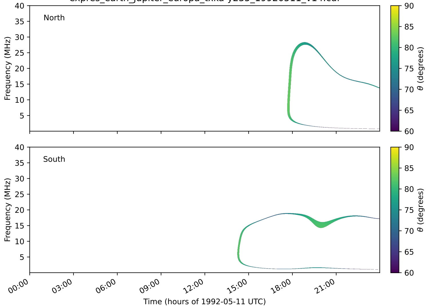
expres_earth_jupiter_europa_txka-y235_19920511_v14.cdf
