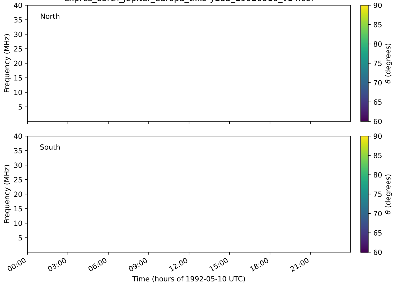
expres_earth_jupiter_europa_txka-y235_19920510_v14.cdf
