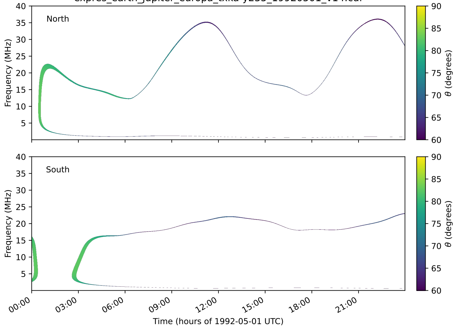
expres_earth_jupiter_europa_txka-y235_19920501_v14.cdf
