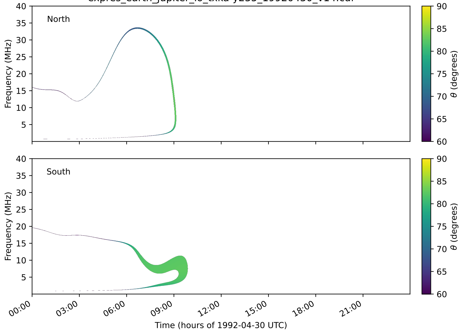
expres_earth_jupiter_io_txka-y235_19920430_v14.cdf
