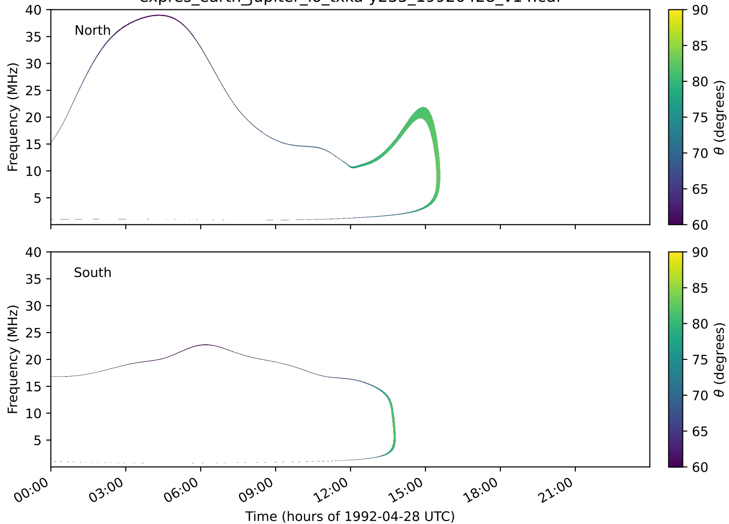
expres_earth_jupiter_io_txka-y235_19920428_v14.cdf
