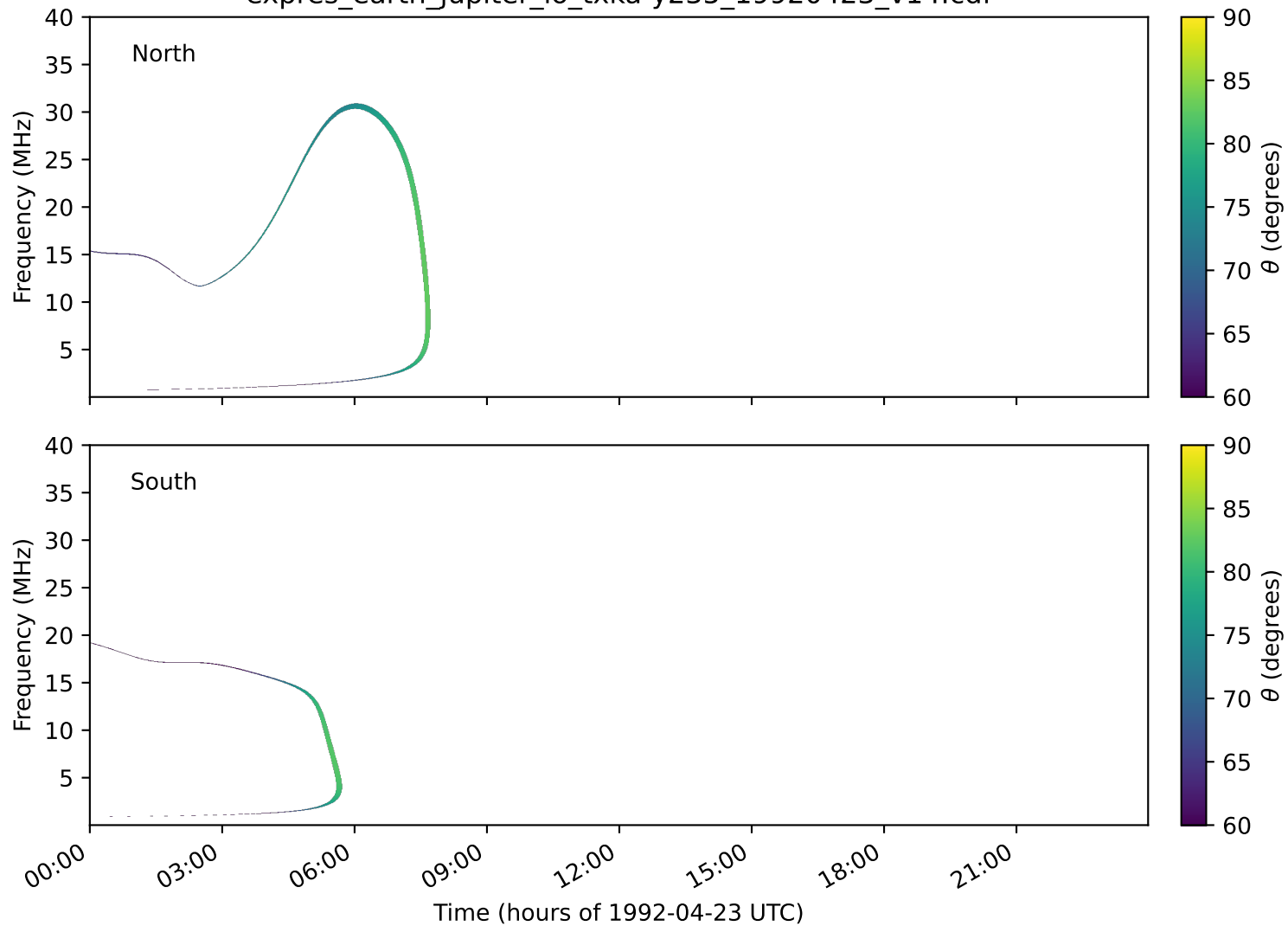
expres_earth_jupiter_io_txka-y235_19920423_v14.cdf
