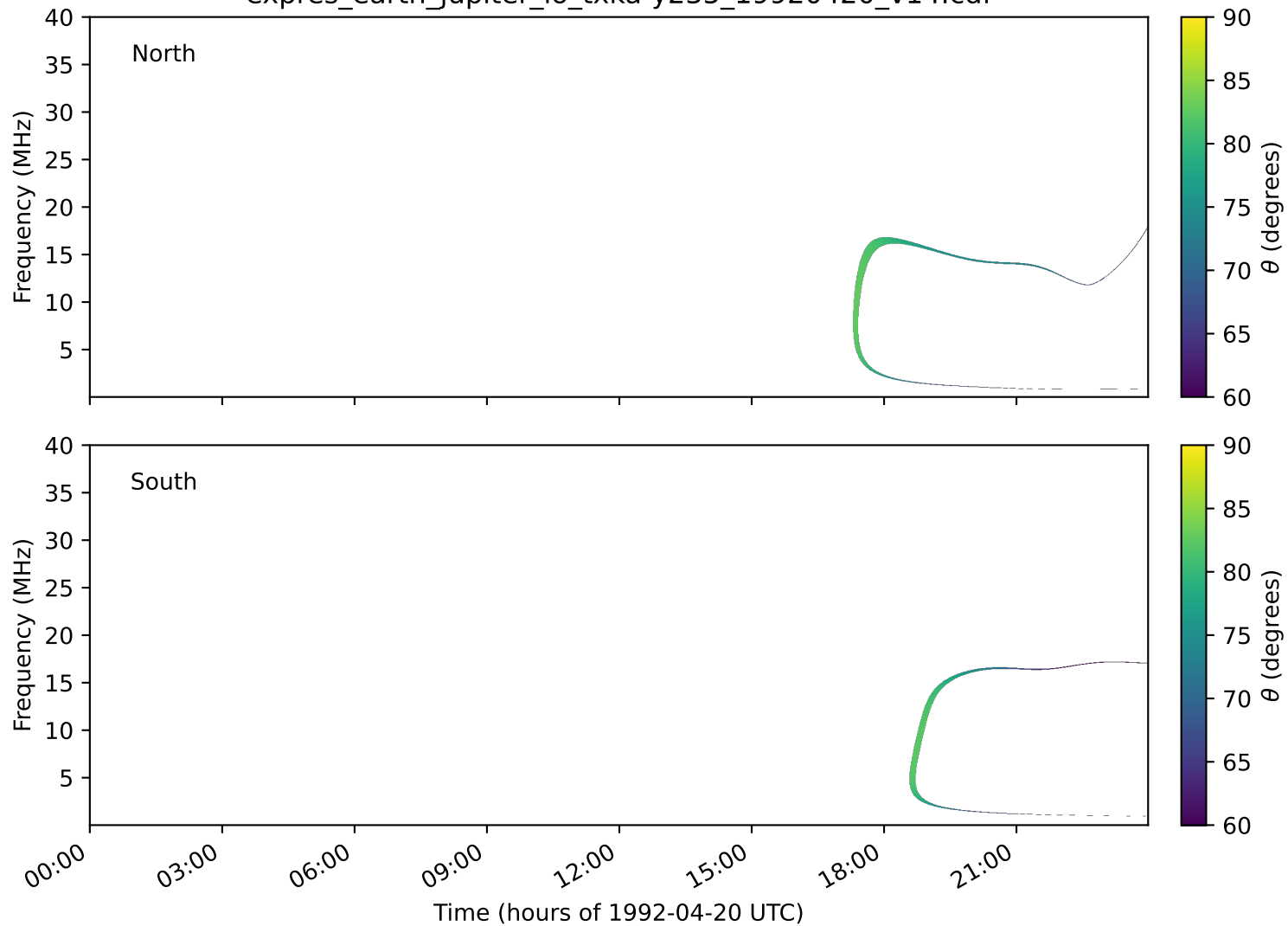
expres_earth_jupiter_io_txka-y235_19920420_v14.cdf
