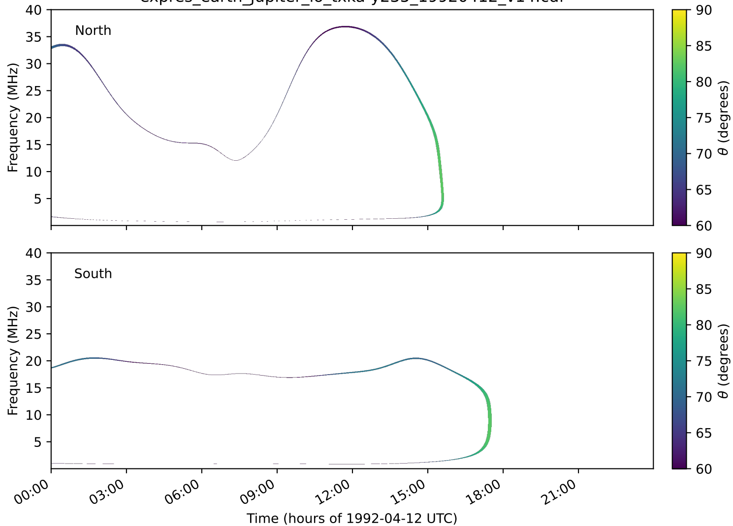
expres_earth_jupiter_io_txka-y235_19920412_v14.cdf
