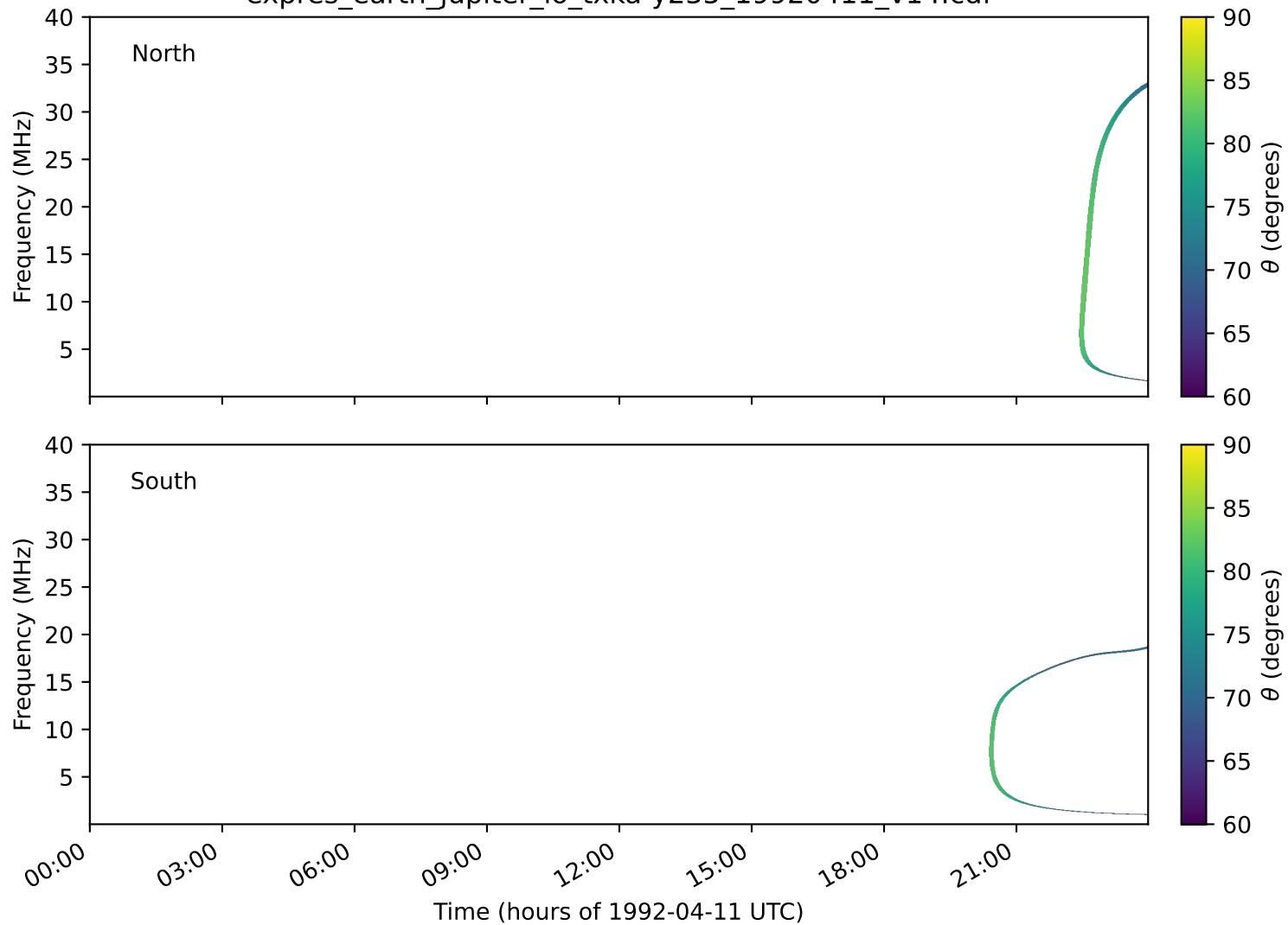
expres_earth_jupiter_io_txka-y235_19920411_v14.cdf
