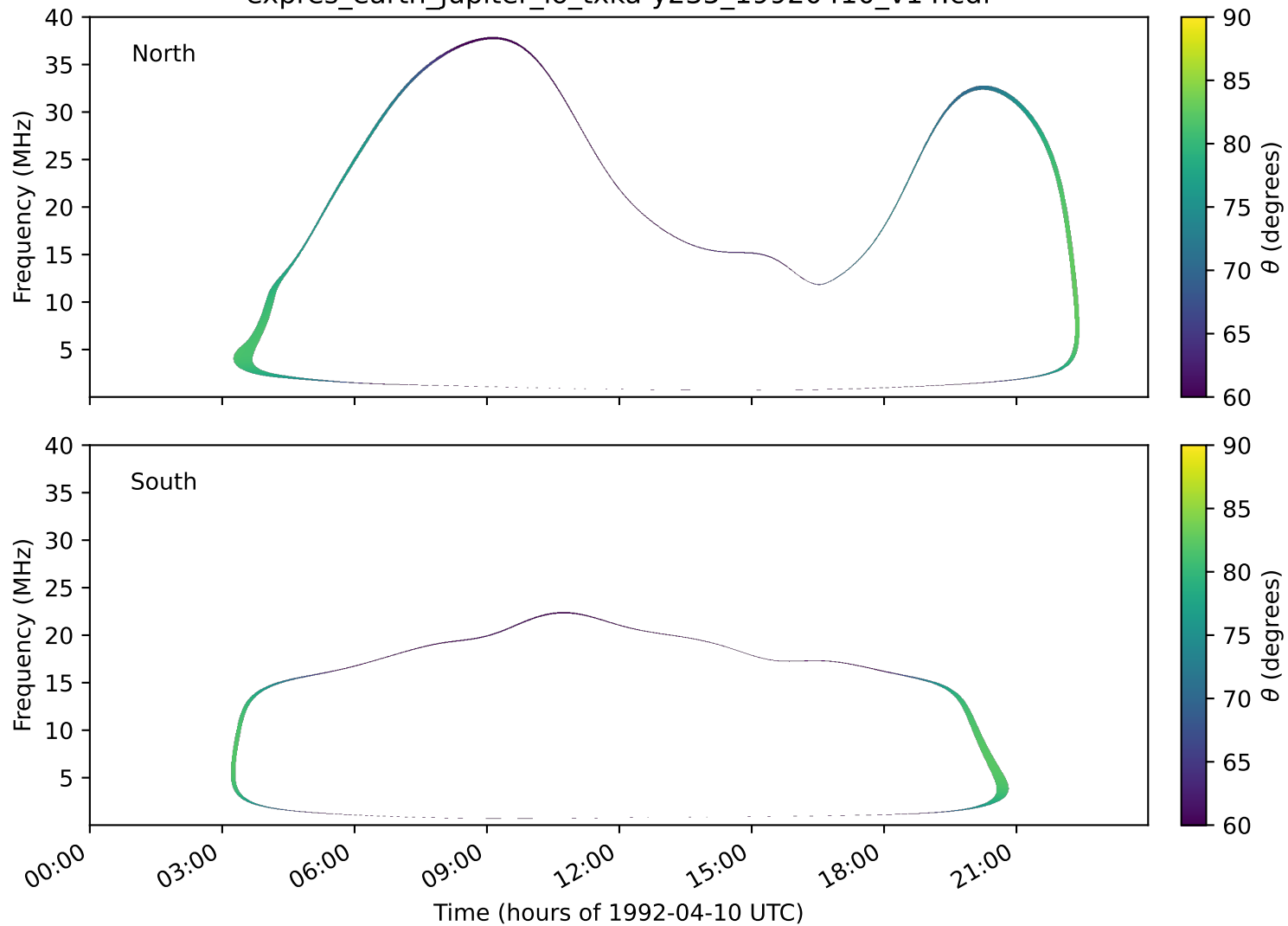
expres_earth_jupiter_io_txka-y235_19920410_v14.cdf
