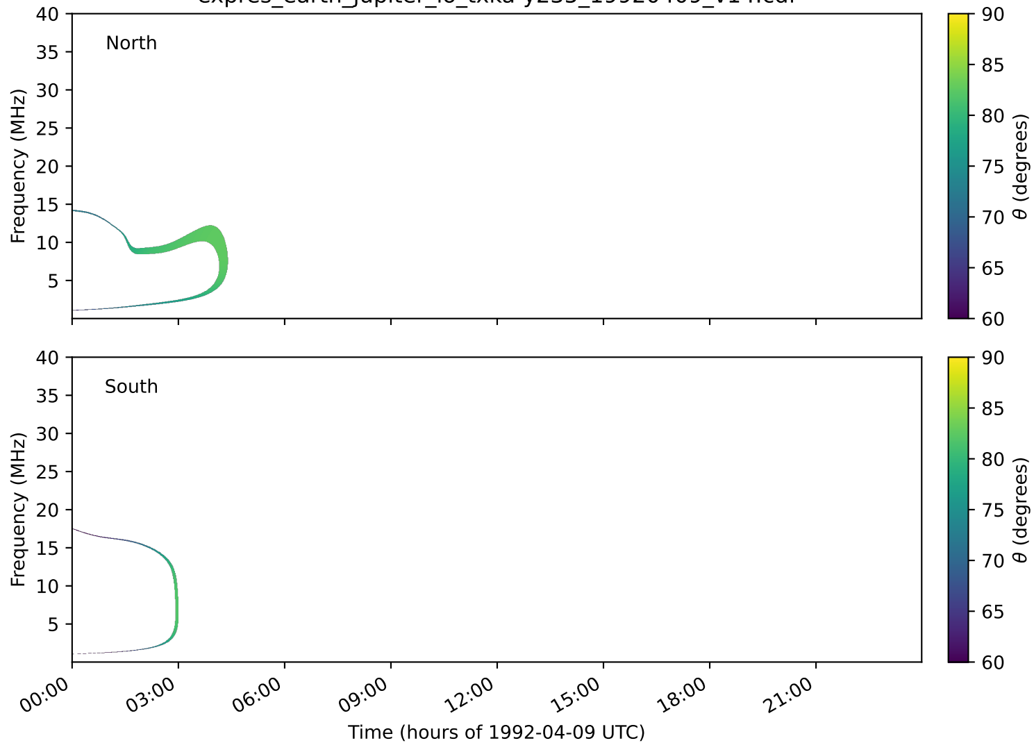
expres_earth_jupiter_io_txka-y235_19920409_v14.cdf
