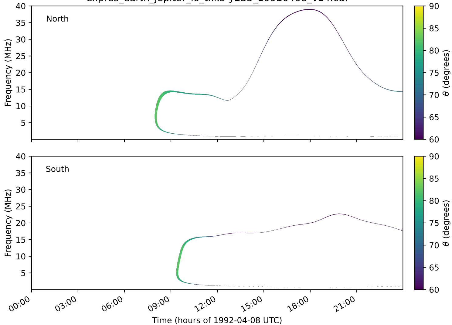
expres_earth_jupiter_io_txka-y235_19920408_v14.cdf
