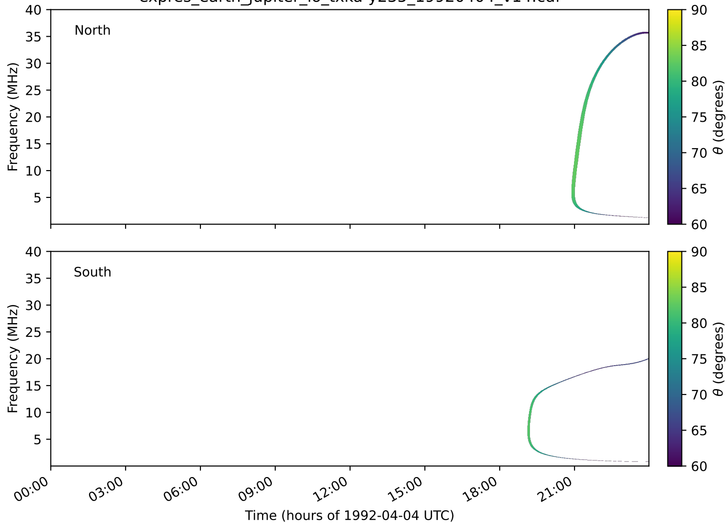
expres_earth_jupiter_io_txka-y235_19920404_v14.cdf
