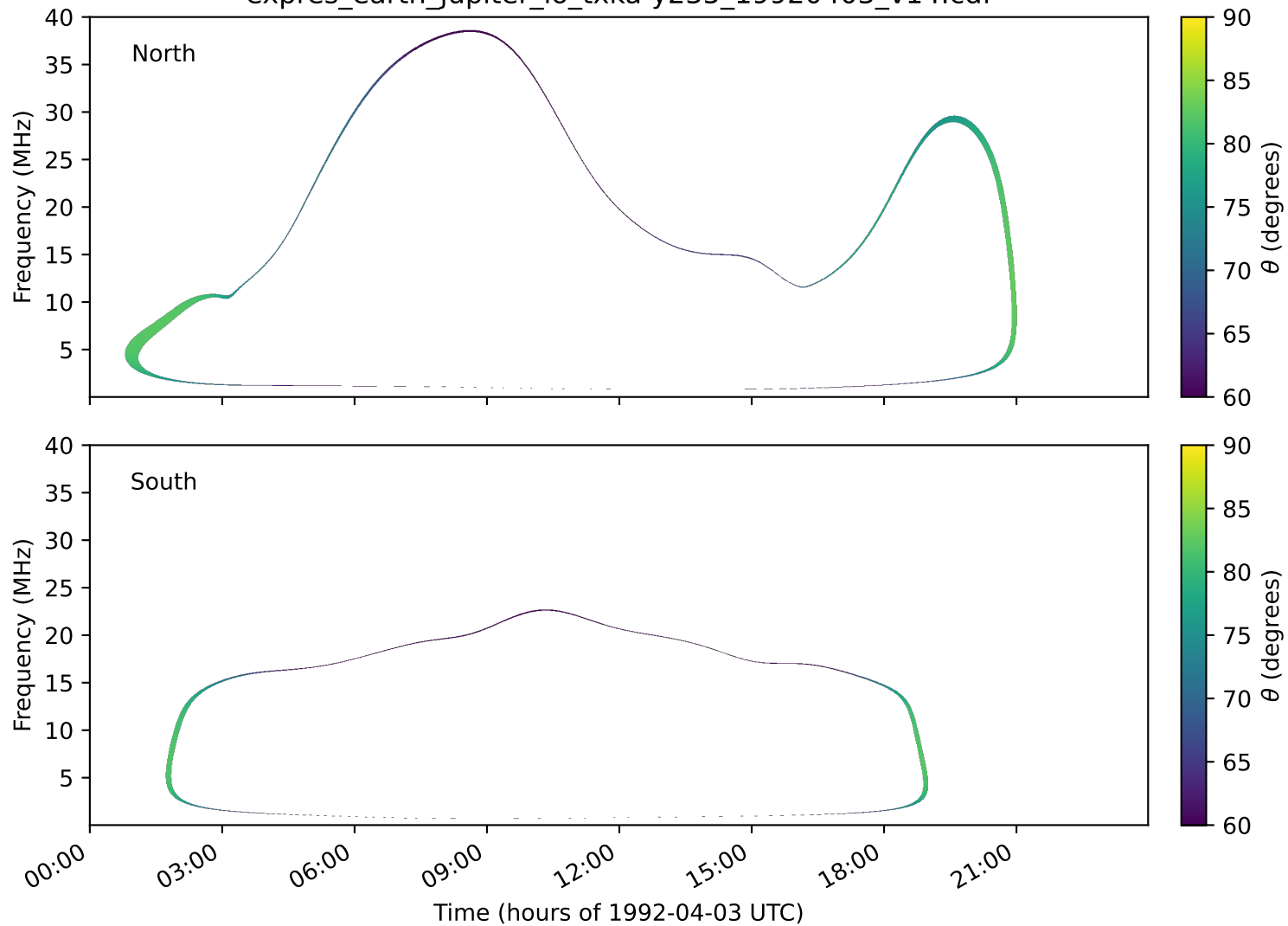
expres_earth_jupiter_io_txka-y235_19920403_v14.cdf
