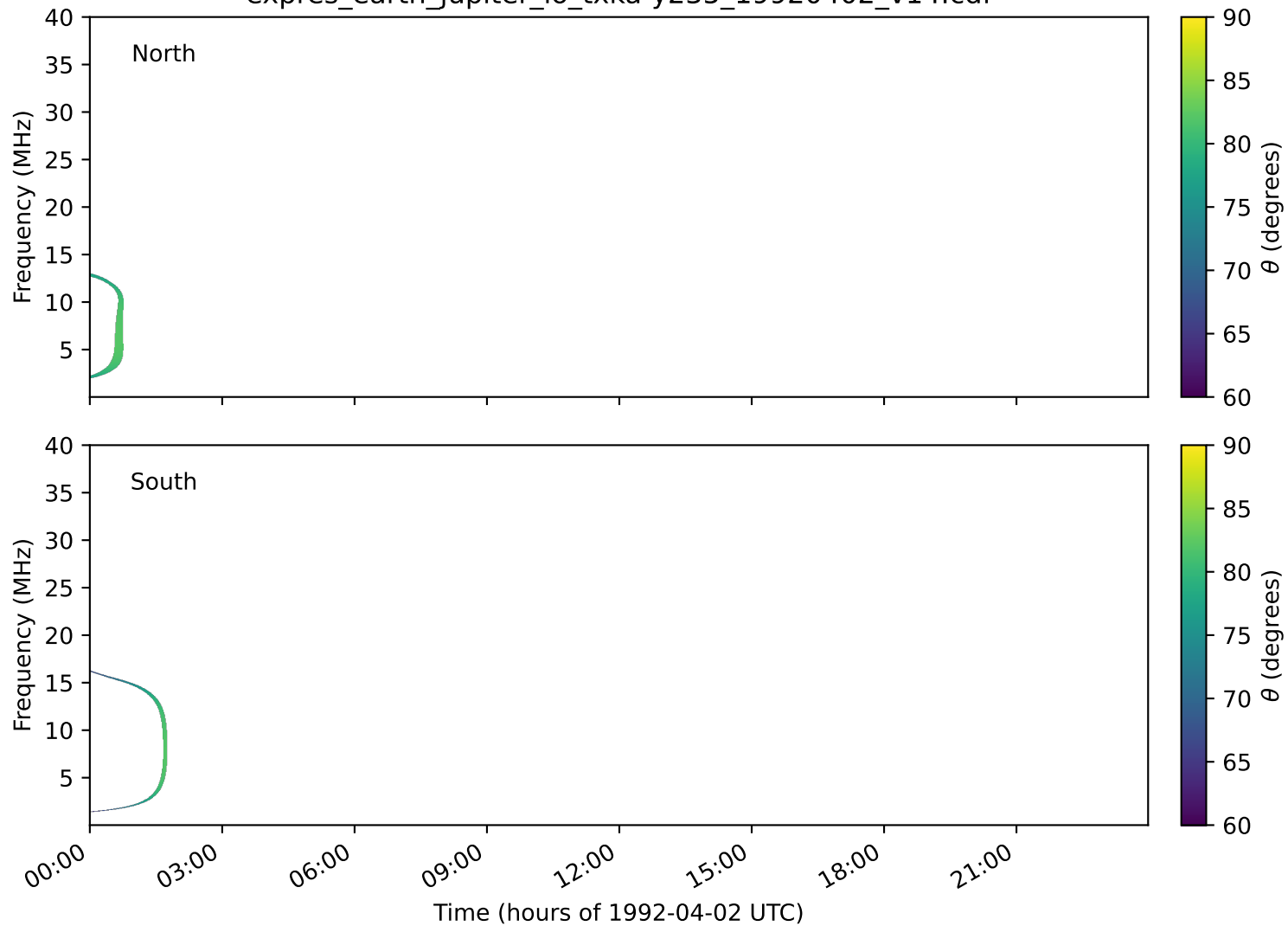
expres_earth_jupiter_io_txka-y235_19920402_v14.cdf
