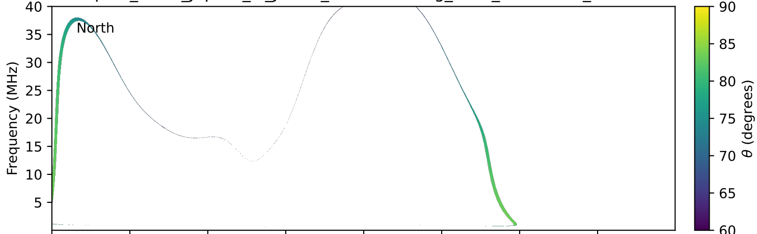
expres_earth_jupiter_io_jrm33_lossc-wid1deg_3kev_19920419_v11.cdf
