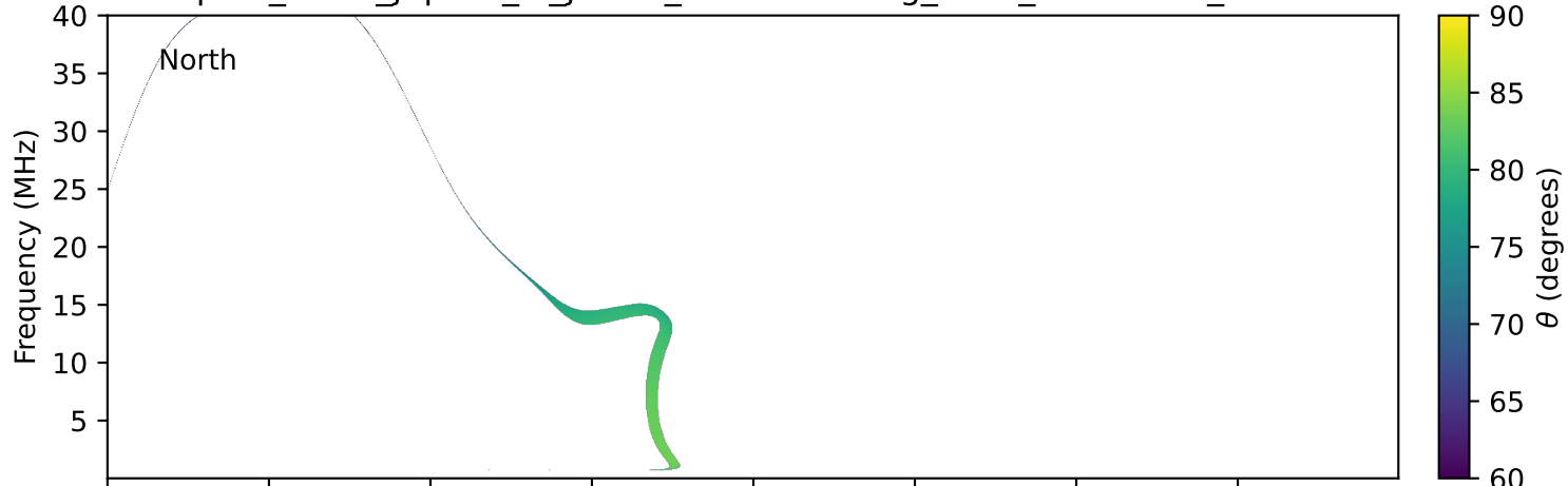
expres_earth_jupiter_io_jrm33_lossc-wid1deg_3kev_19920414_v11.cdf
