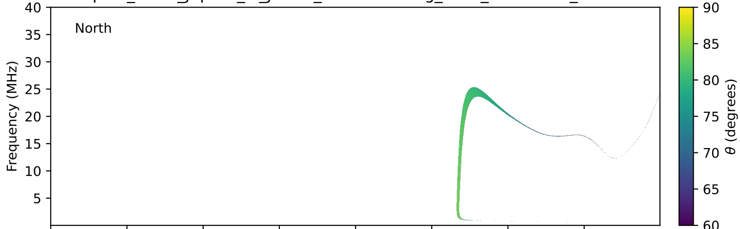
expres_earth_jupiter_io_jrm33_lossc-wid1deg_3kev_19920413_v11.cdf
