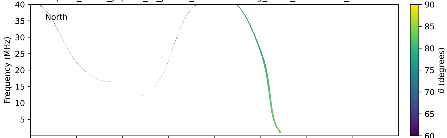
expres_earth_jupiter_io_jrm33_lossc-wid1deg_3kev_19920412_v11.cdf
