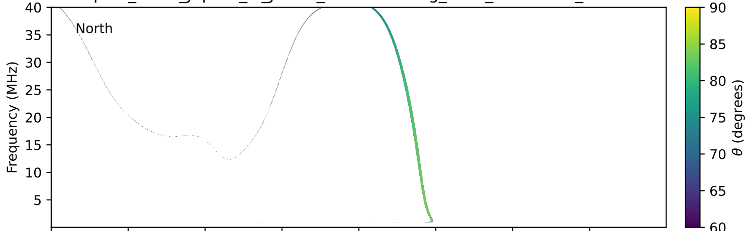
expres_earth_jupiter_io_jrm33_lossc-wid1deg_3kev_19920405_v11.cdf
