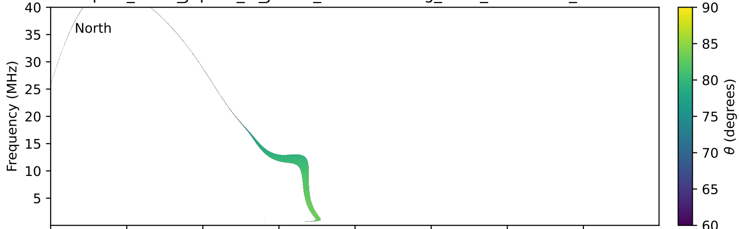
expres_earth_jupiter_io_jrm09_lossc-wid1deg_3kev_19920414_v11.cdf
