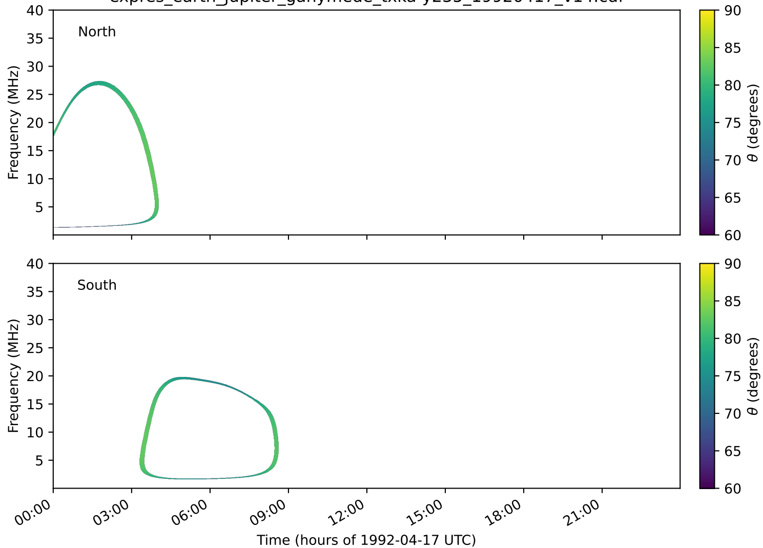
expres_earth_jupiter_ganymede_txka-y235_19920417_v14.cdf
