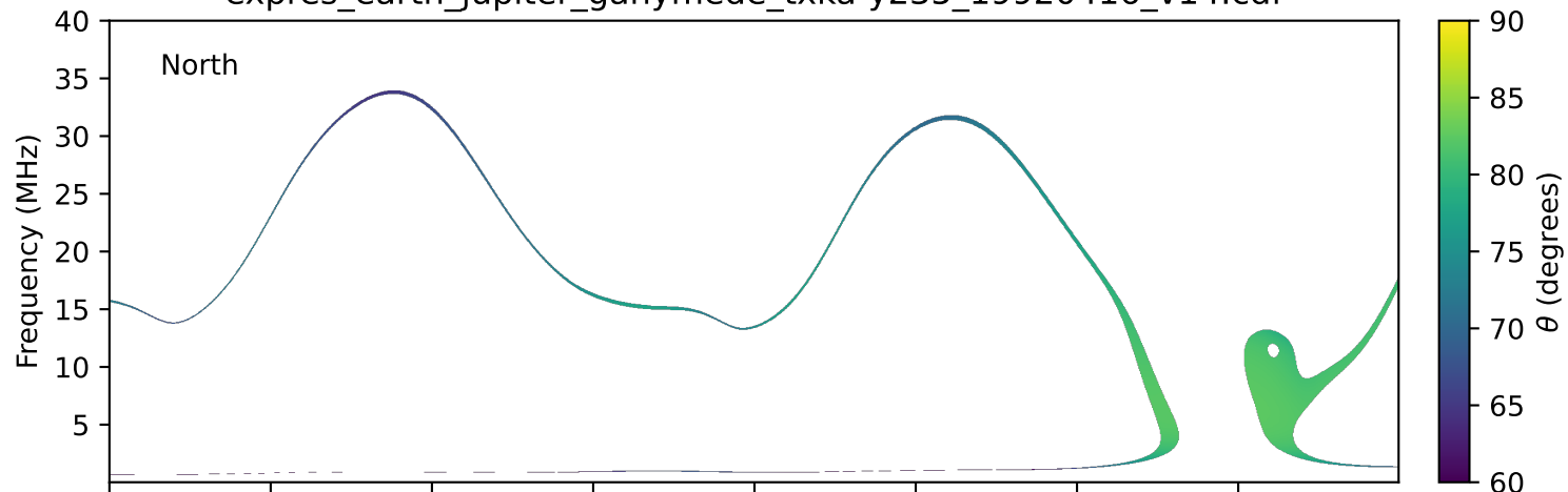
expres_earth_jupiter_ganymede_txka-y235_19920416_v14.cdf
