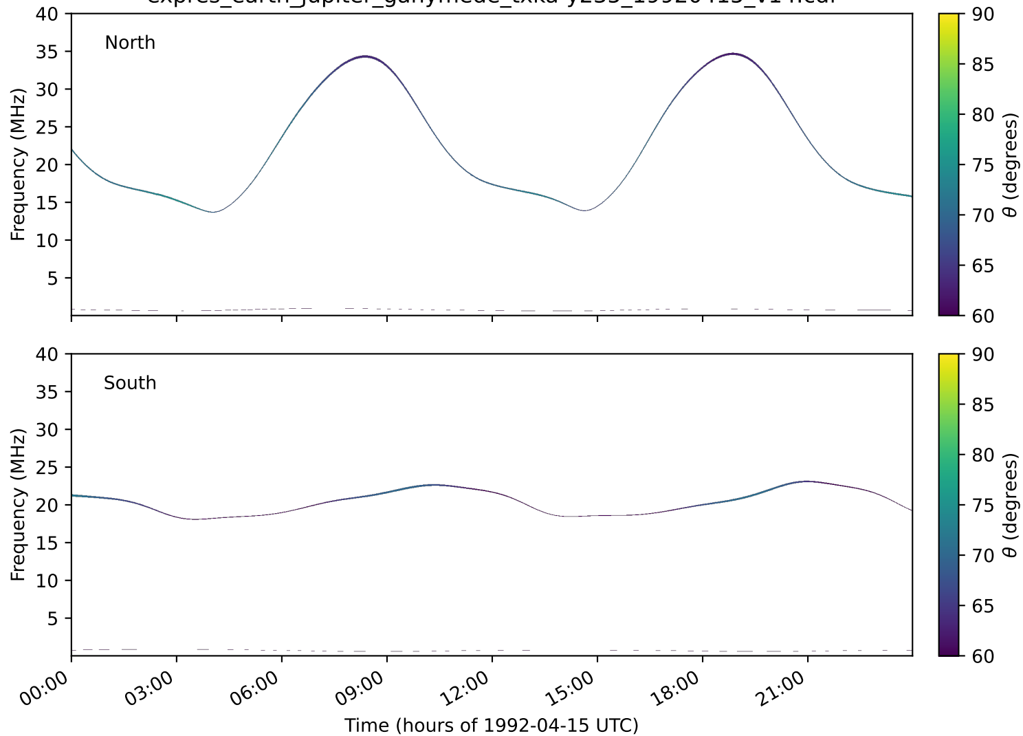
expres_earth_jupiter_ganymede_txka-y235_19920415_v14.cdf
