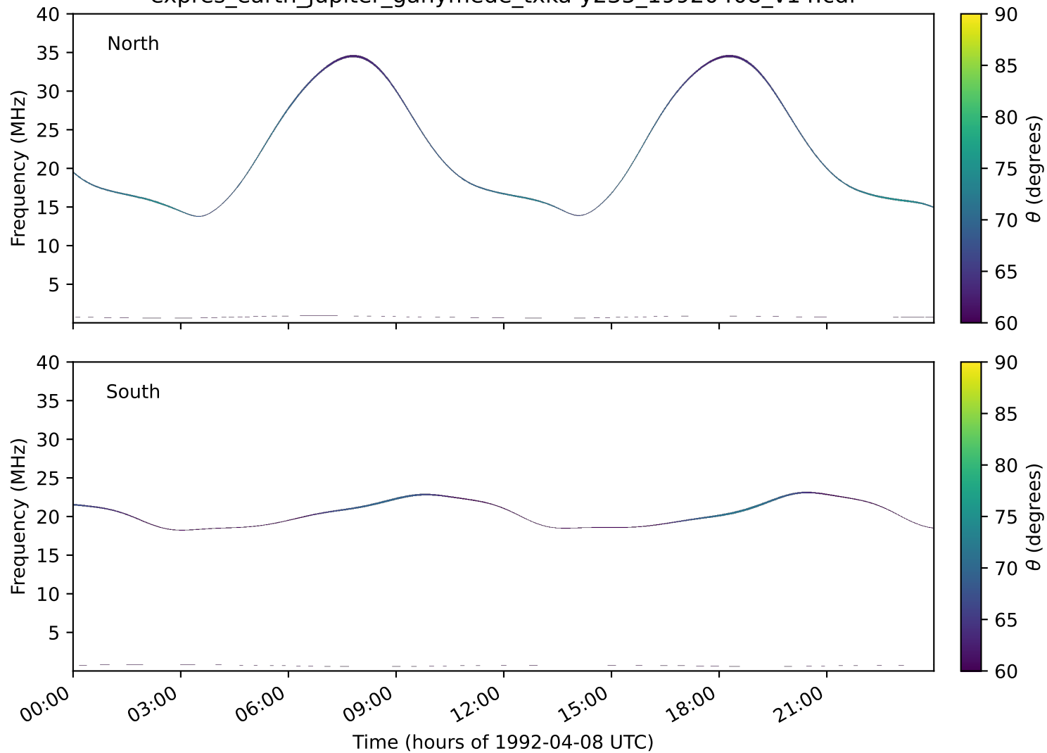
expres_earth_jupiter_ganymede_txka-y235_19920408_v14.cdf
