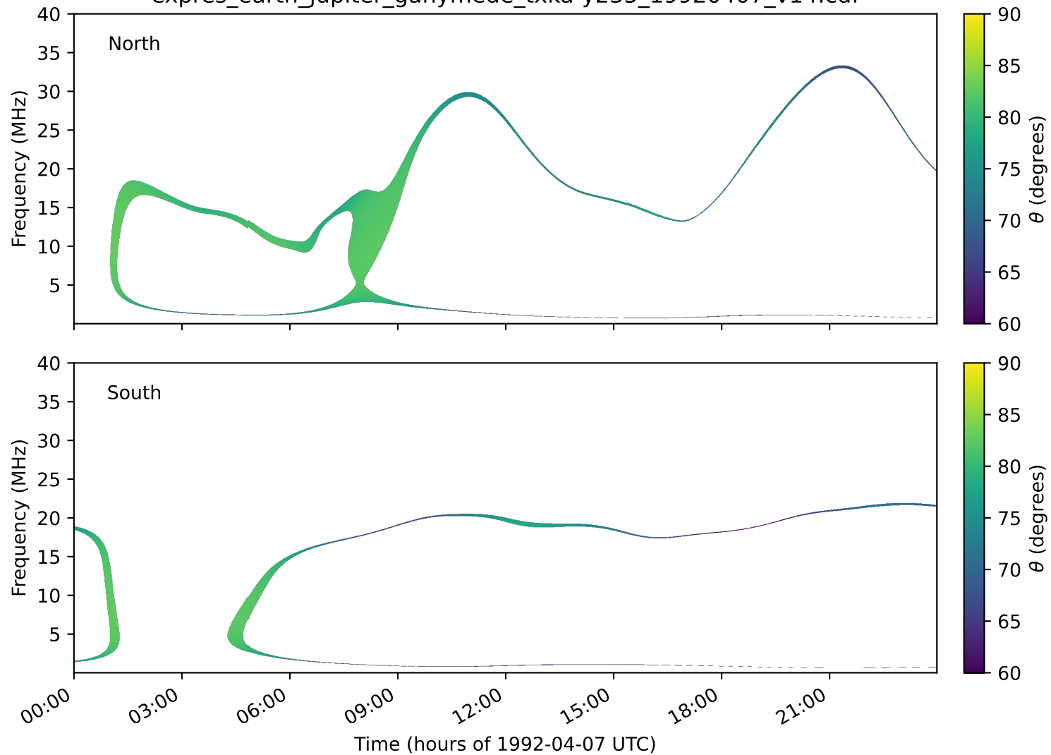
expres_earth_jupiter_ganymede_txka-y235_19920407_v14.cdf
