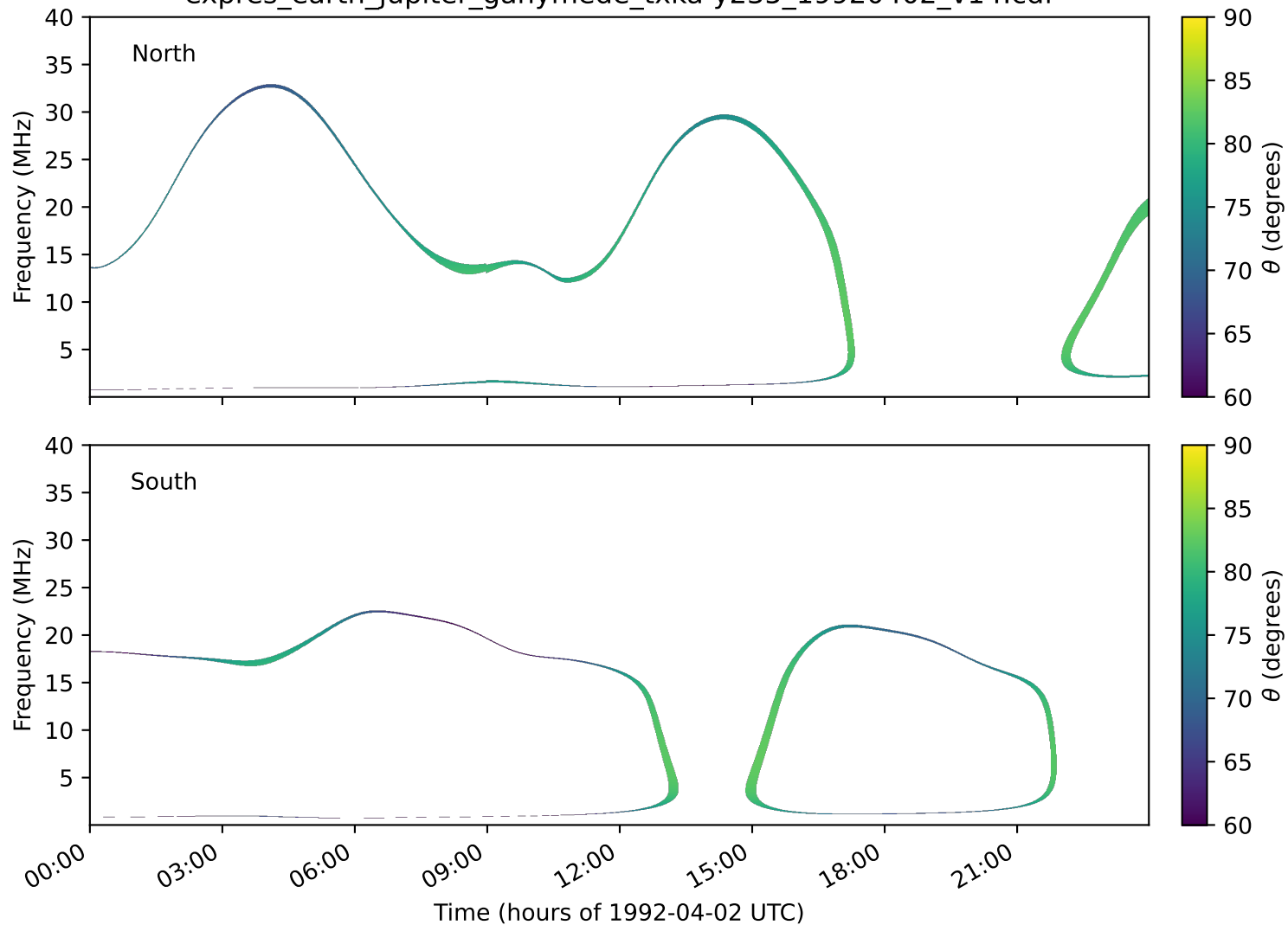
expres_earth_jupiter_ganymede_txka-y235_19920402_v14.cdf
