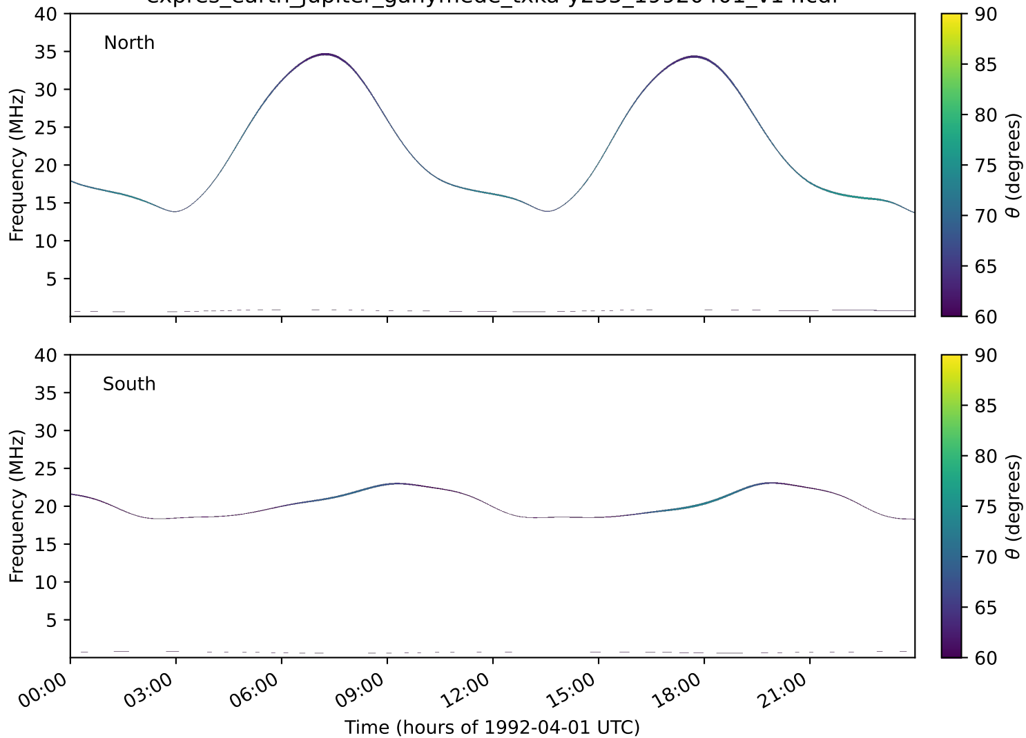
expres_earth_jupiter_ganymede_txka-y235_19920401_v14.cdf
