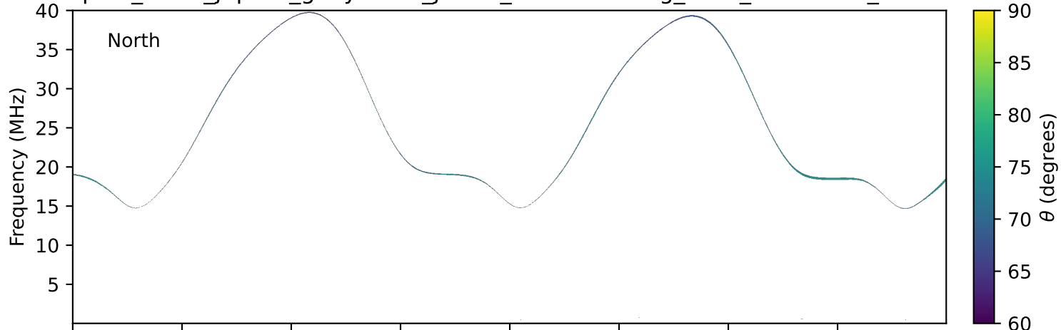
expres_earth_jupiter_ganymede_jrm33_lossc-wid1deg_3kev_19920430_v11.cdf
