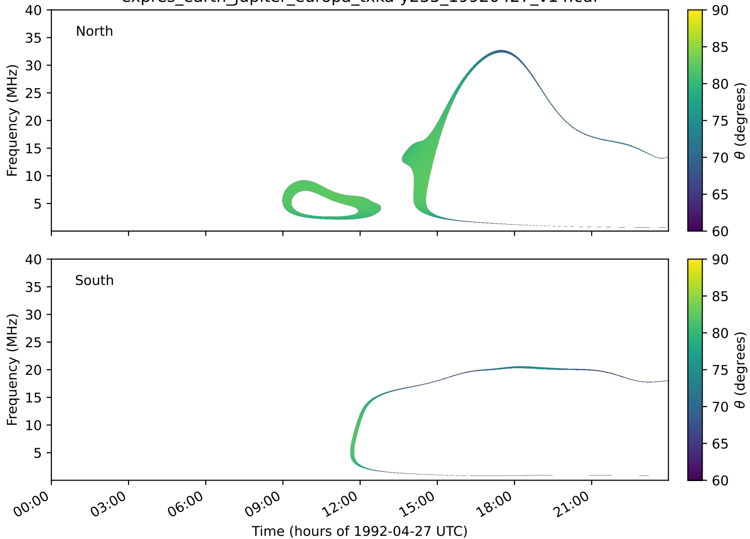
expres_earth_jupiter_europa_txka-y235_19920427_v14.cdf
