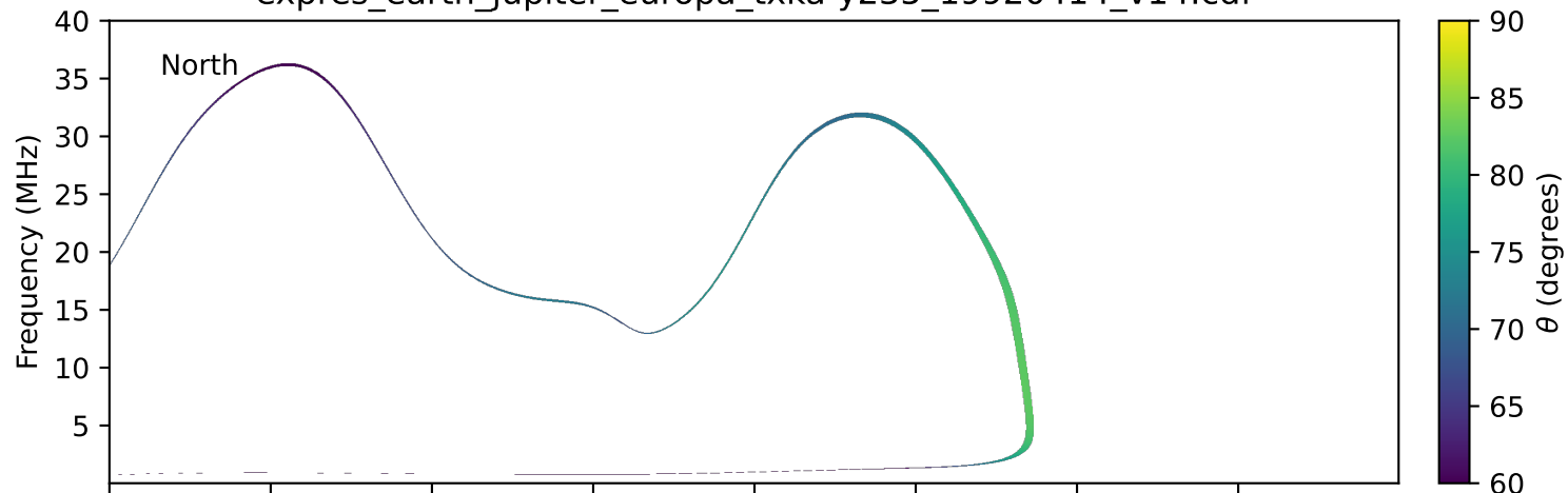
expres_earth_jupiter_europa_txka-y235_19920414_v14.cdf
