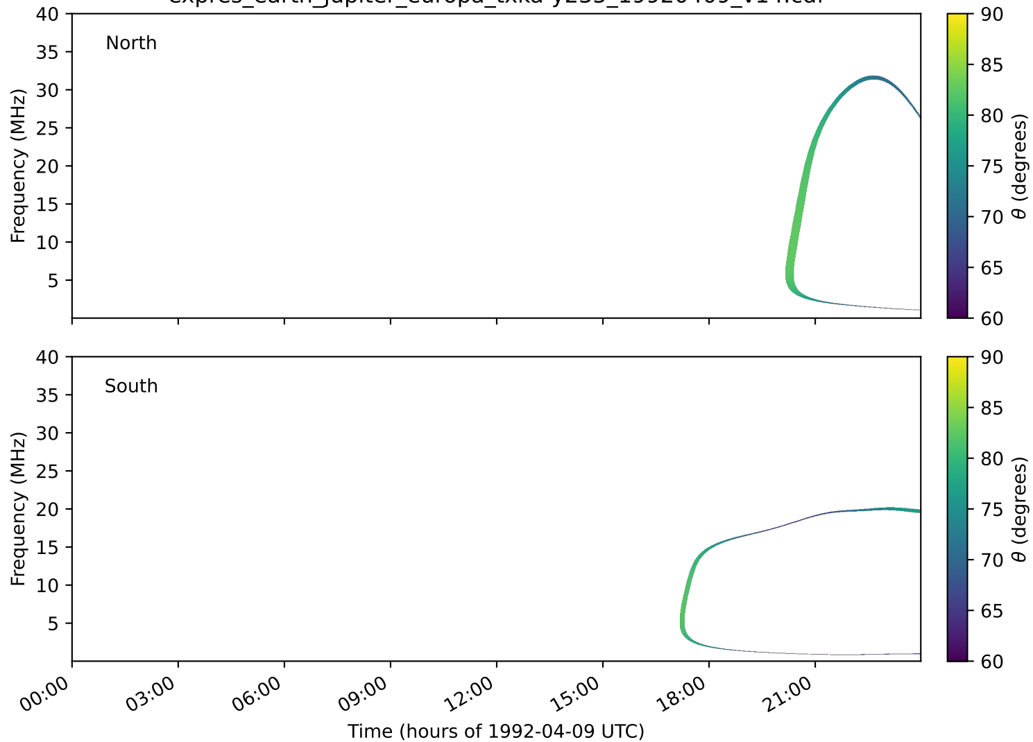
expres_earth_jupiter_europa_txka-y235_19920409_v14.cdf
