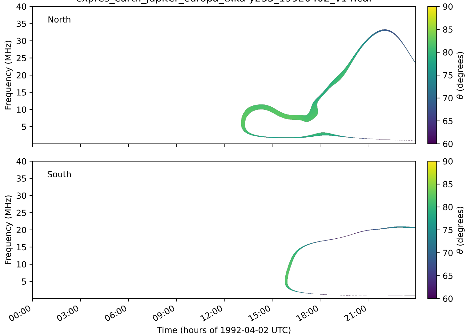
expres_earth_jupiter_europa_txka-y235_19920402_v14.cdf
