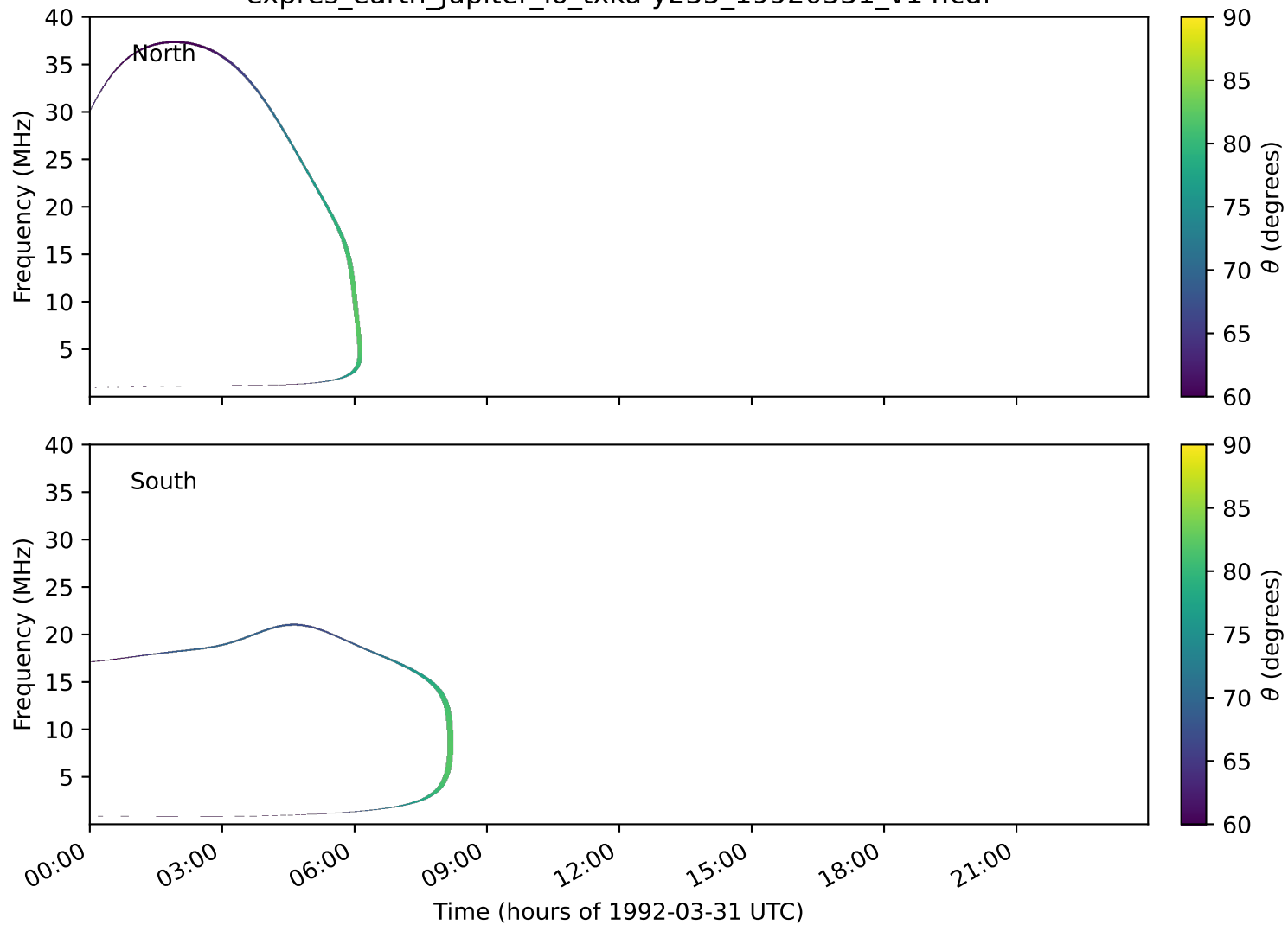
expres_earth_jupiter_io_txka-y235_19920331_v14.cdf
