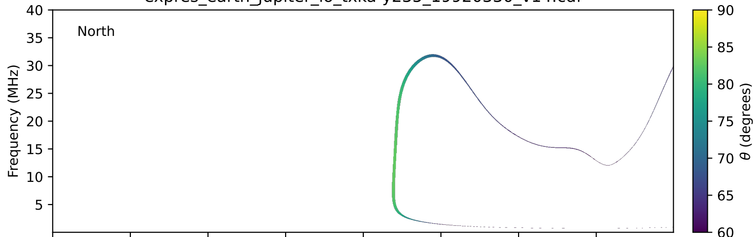
expres_earth_jupiter_io_txka-y235_19920330_v14.cdf
