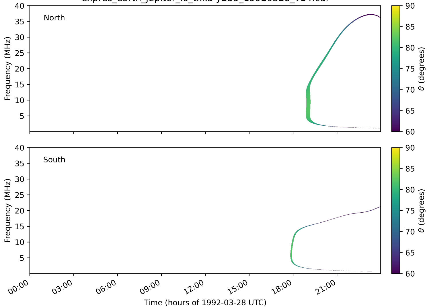
expres_earth_jupiter_io_txka-y235_19920328_v14.cdf
