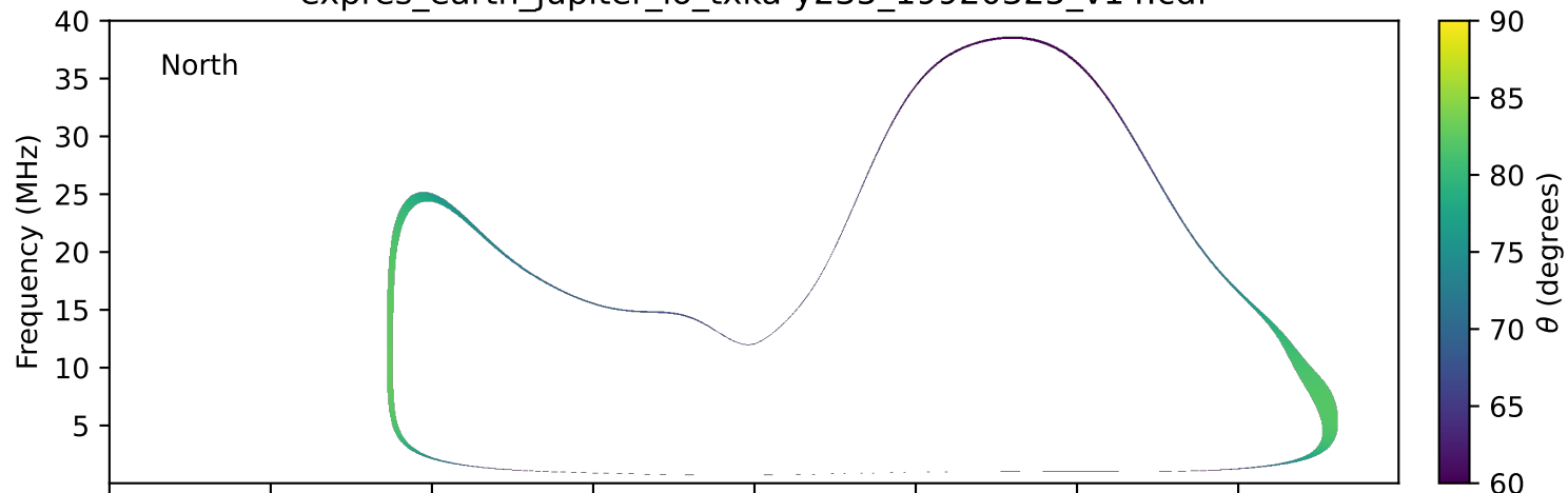
expres_earth_jupiter_io_txka-y235_19920325_v14.cdf
