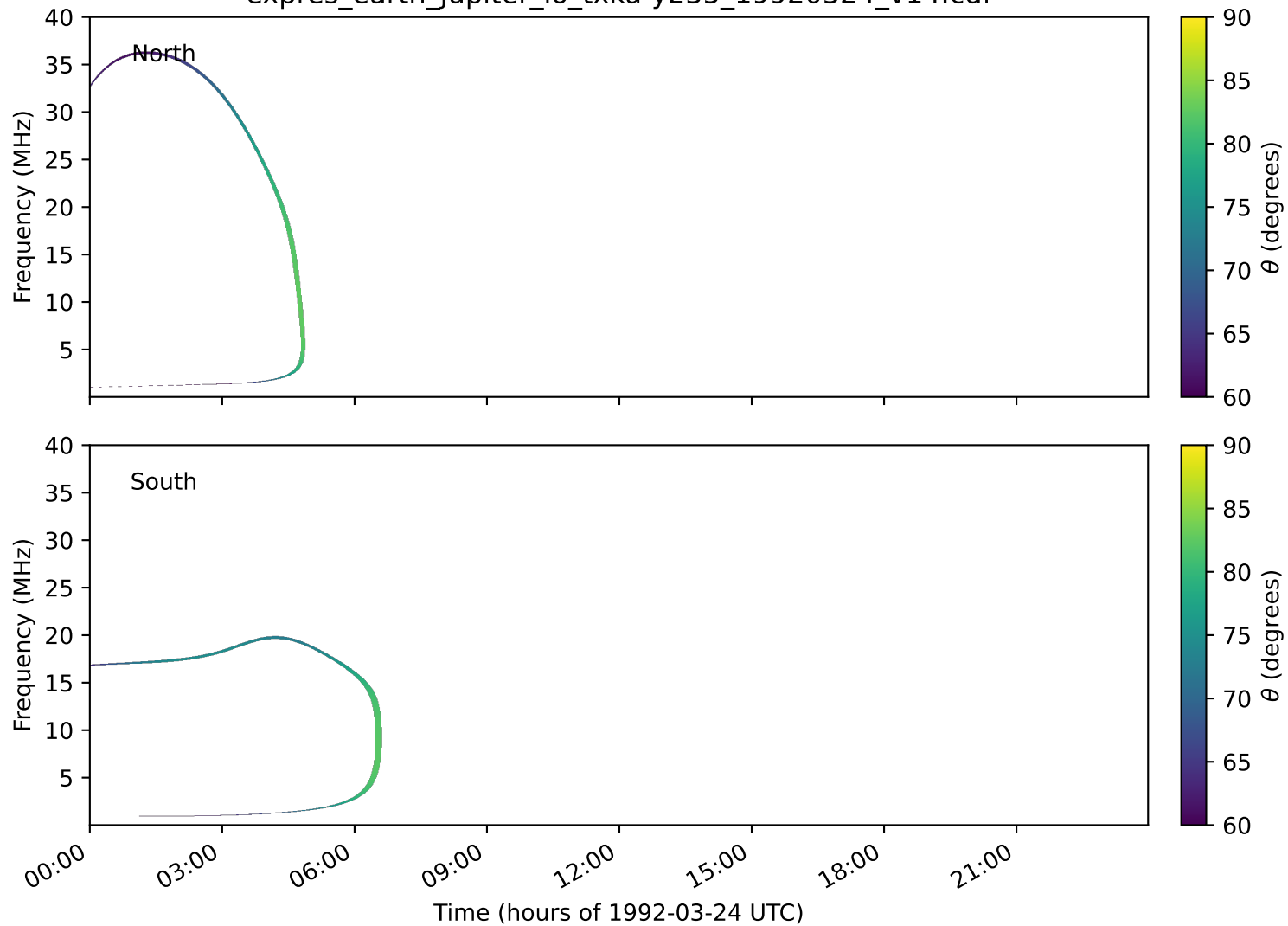
expres_earth_jupiter_io_txka-y235_19920324_v14.cdf
