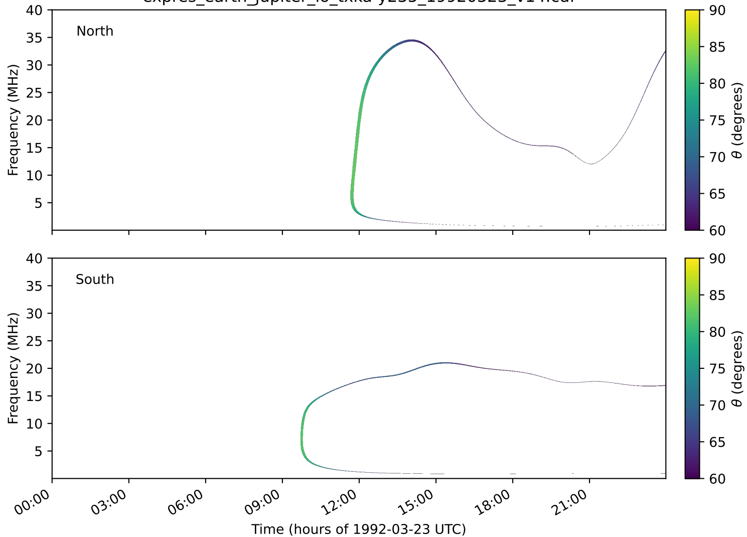
expres_earth_jupiter_io_txka-y235_19920323_v14.cdf
