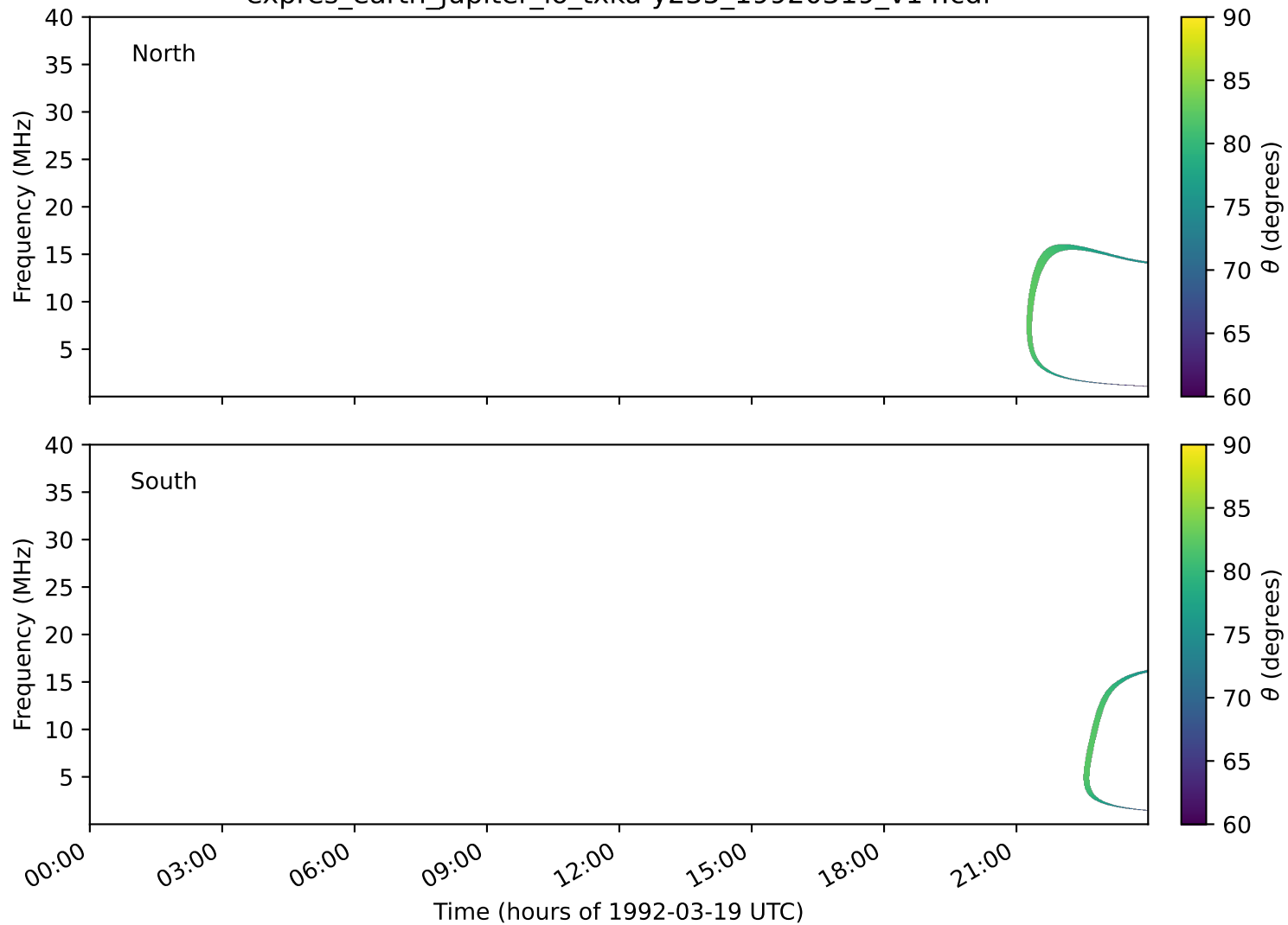
expres_earth_jupiter_io_txka-y235_19920319_v14.cdf
