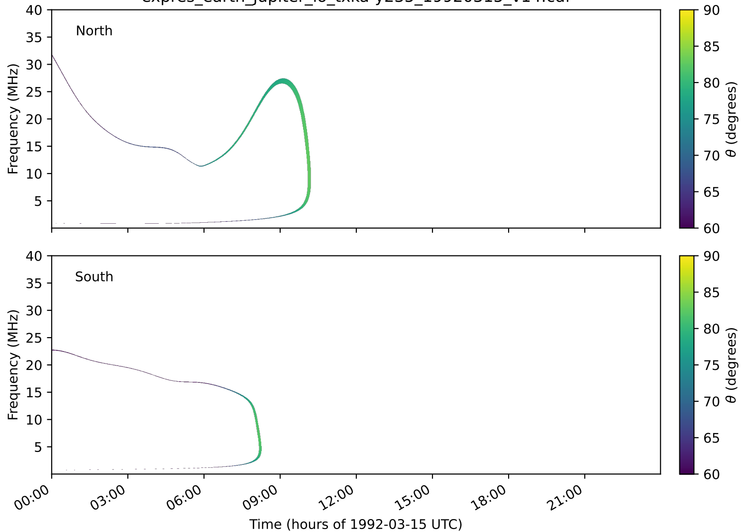
expres_earth_jupiter_io_txka-y235_19920315_v14.cdf
