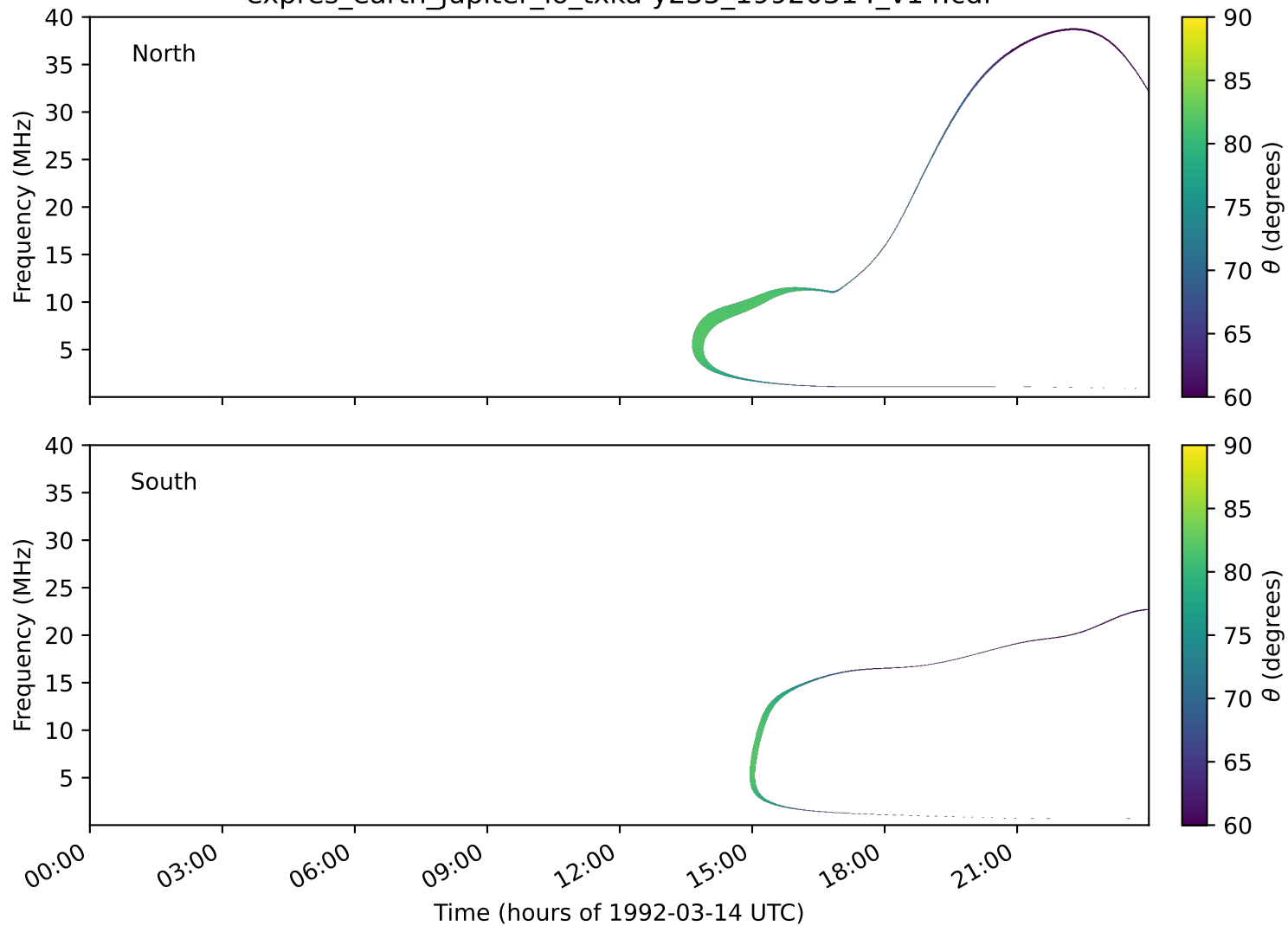
expres_earth_jupiter_io_txka-y235_19920314_v14.cdf
