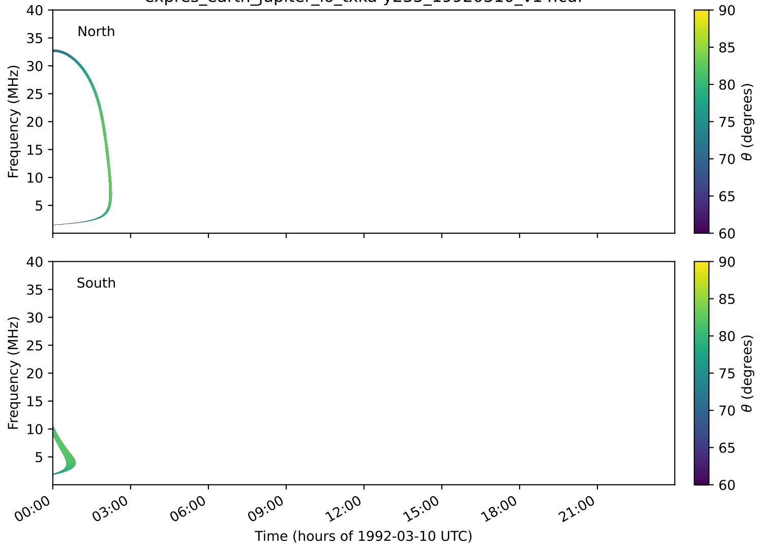
expres_earth_jupiter_io_txka-y235_19920310_v14.cdf
