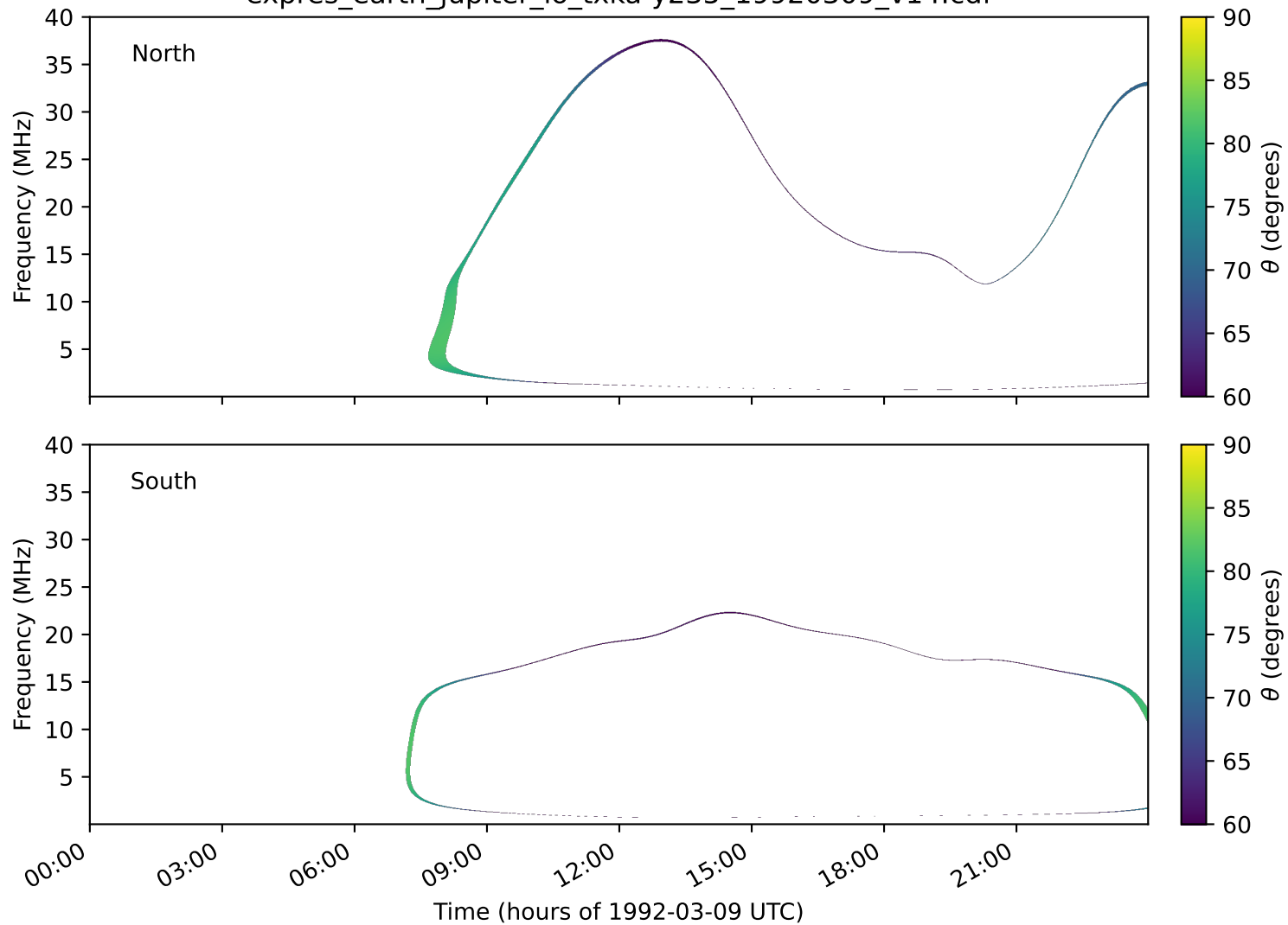
expres_earth_jupiter_io_txka-y235_19920309_v14.cdf
